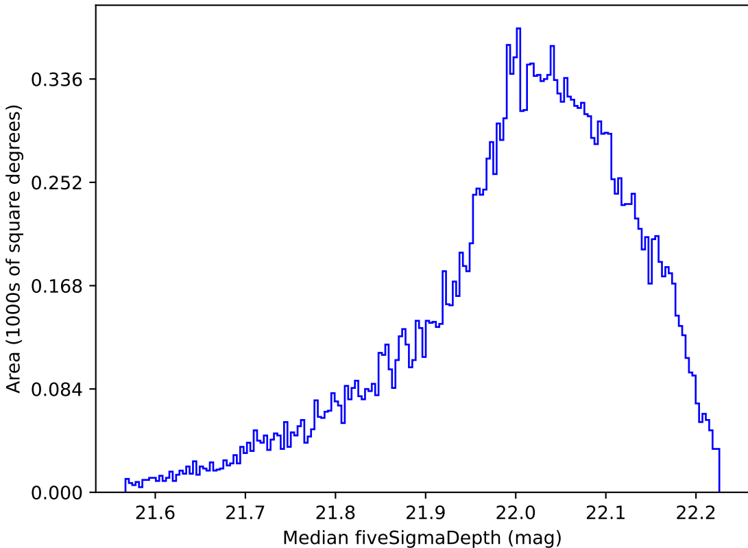
no_magell_roll_v3.4_10yrs All sky y band: Median fiveSigmaDepth
