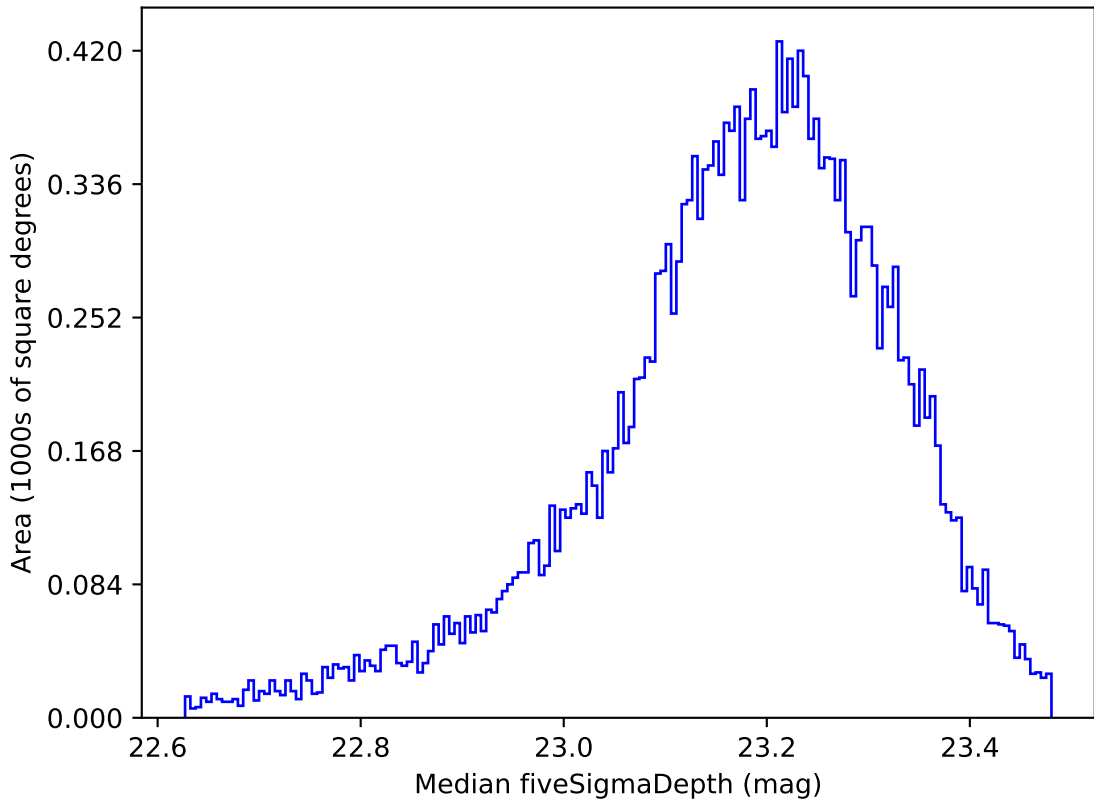
no_magell_roll_v3.4_10yrs All sky u band: Median fiveSigmaDepth
