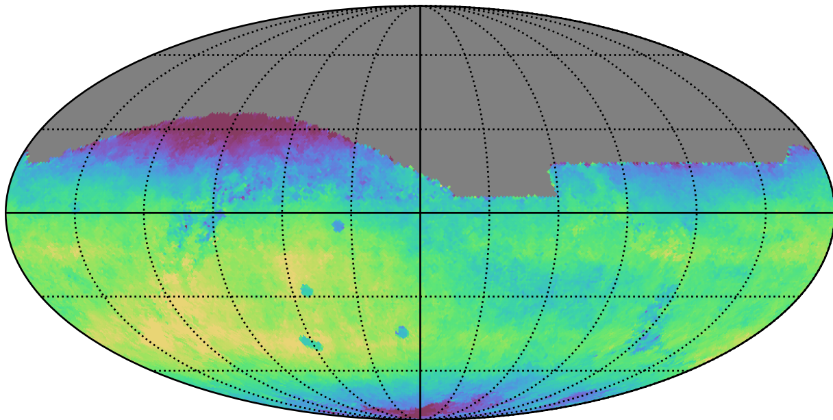
no_magell_roll_v3.4_10yrs All sky r band: Median fiveSigmaDepth
