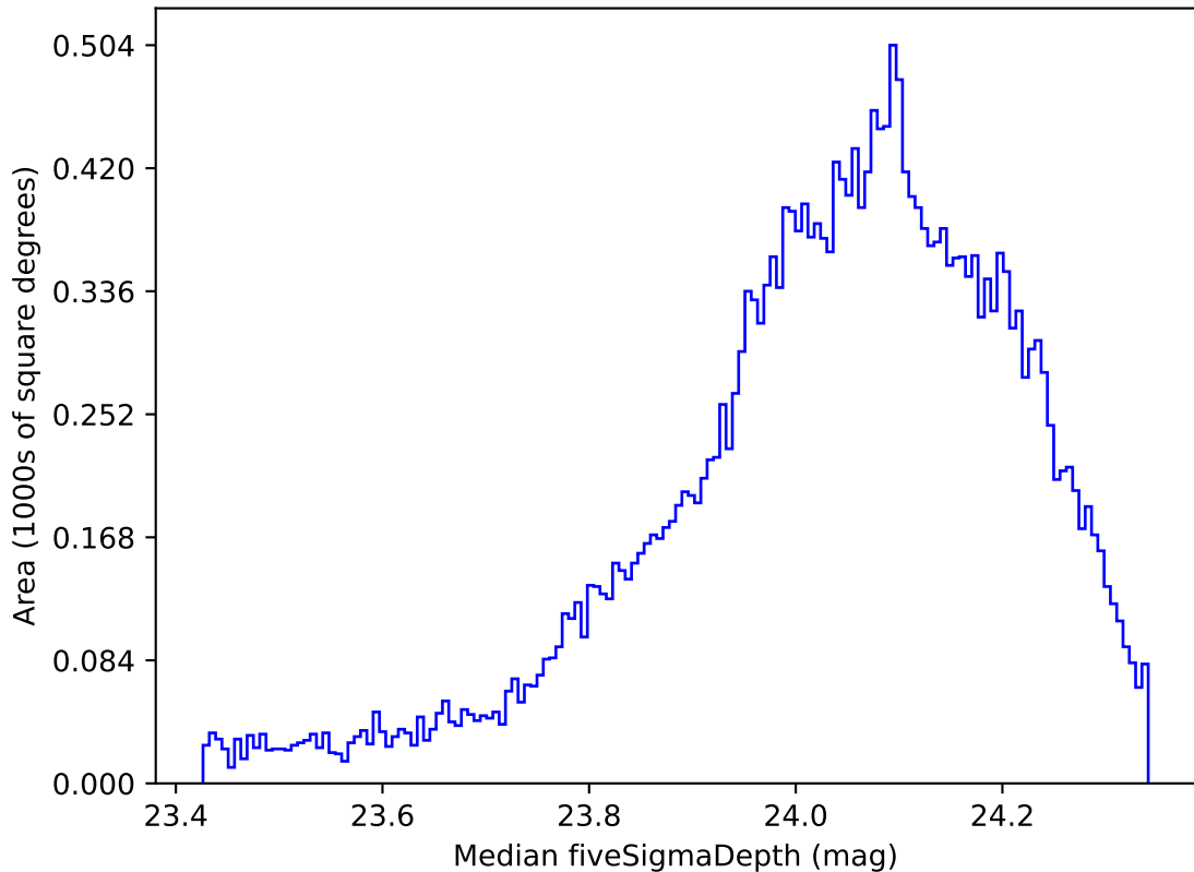
no_magell_roll_v3.4_10yrs All sky r band: Median fiveSigmaDepth
