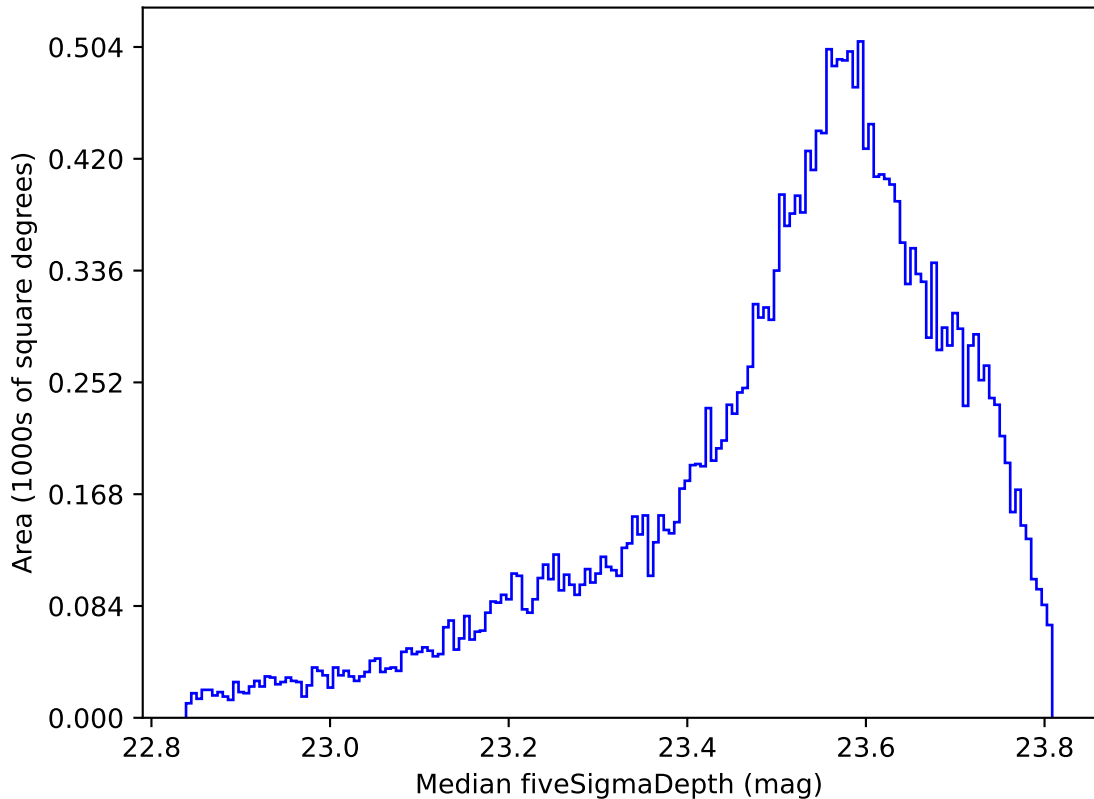
no_magell_roll_v3.4_10yrs All sky i band: Median fiveSigmaDepth
