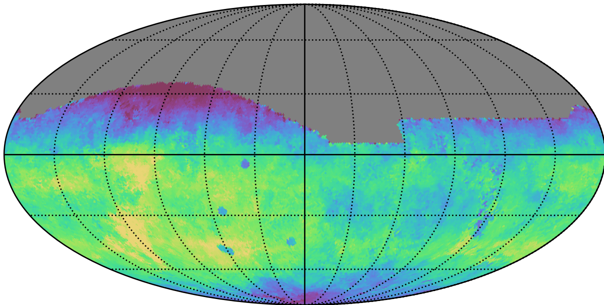
no_magell_roll_v3.4_10yrs All sky g band: Median fiveSigmaDepth
