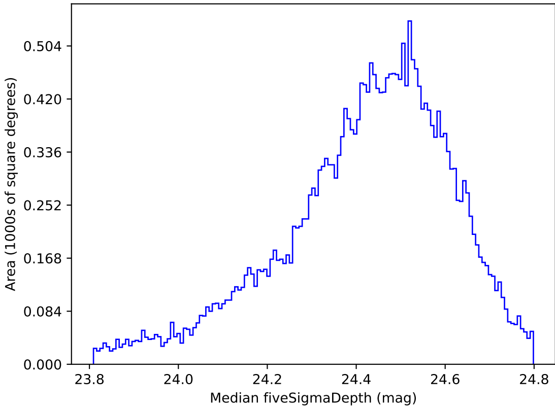
no_magell_roll_v3.4_10yrs All sky g band: Median fiveSigmaDepth
