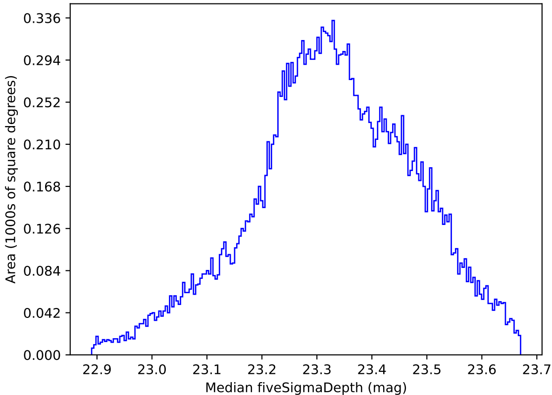
no_magell_roll_v3.4_10yrs All sky all bands: Median fiveSigmaDepth
