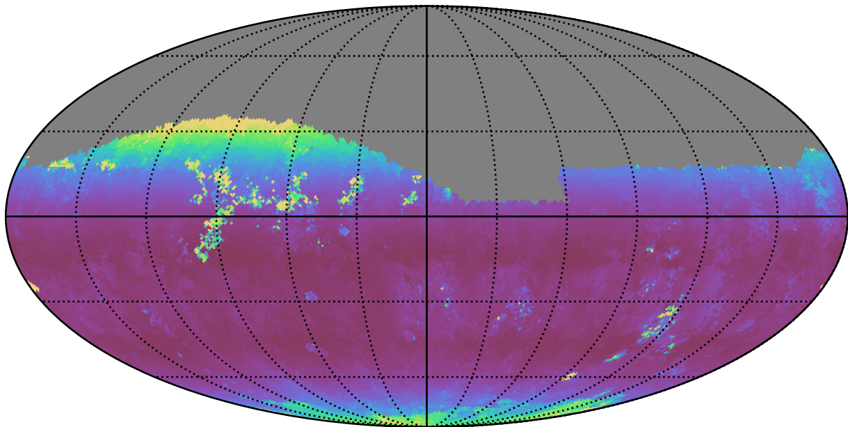
no_magell_roll_v3.4_10yrs Yr 1 z band: Median airmass
