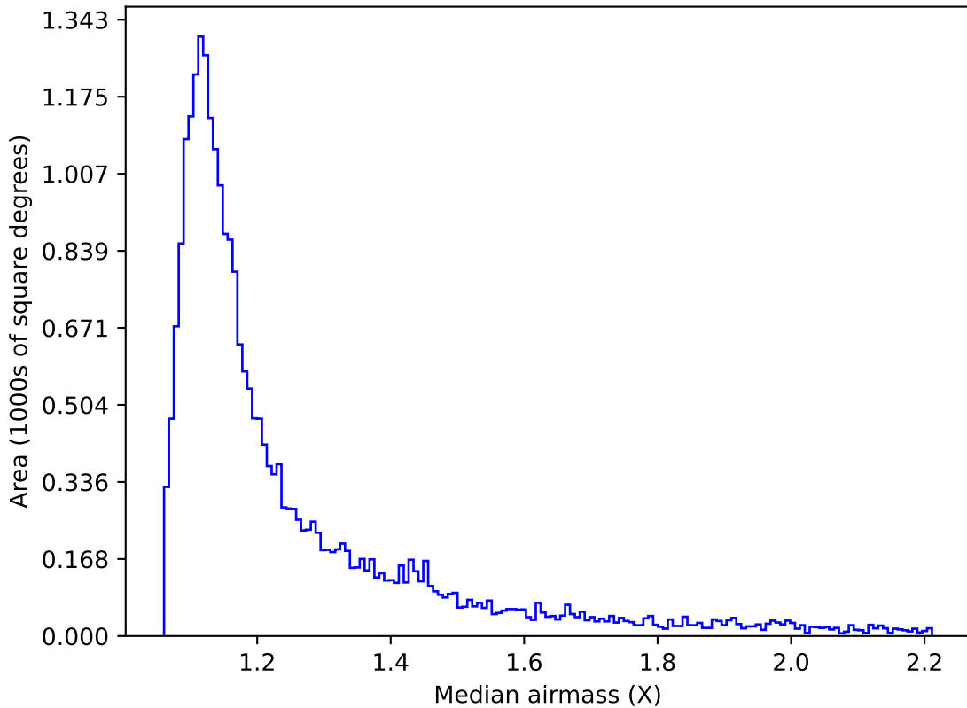
no_magell_roll_v3.4_10yrs Yr 1 z band: Median airmass
