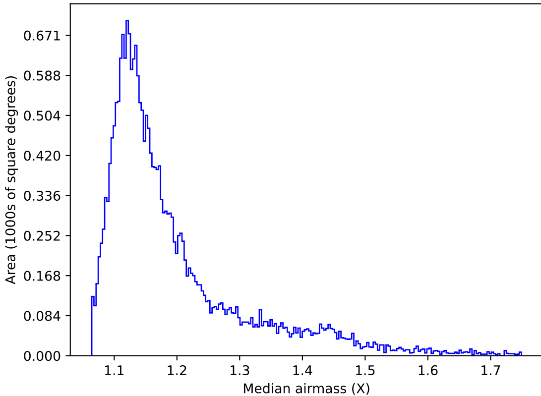
no_magell_roll_v3.4_10yrs Yr 1 y band: Median airmass
