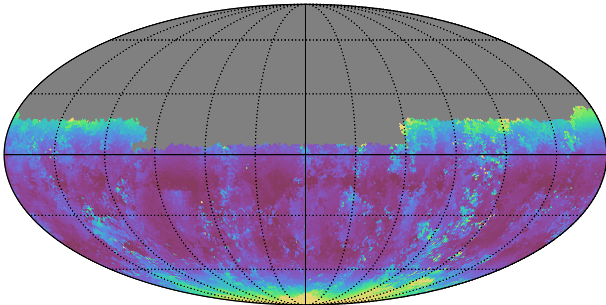
no_magell_roll_v3.4_10yrs Yr 1 u band: Median airmass
