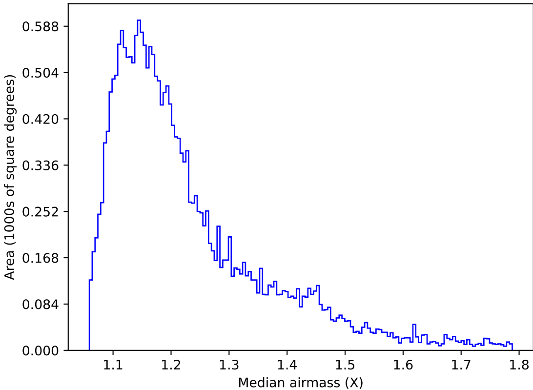
no_magell_roll_v3.4_10yrs Yr 1 u band: Median airmass
