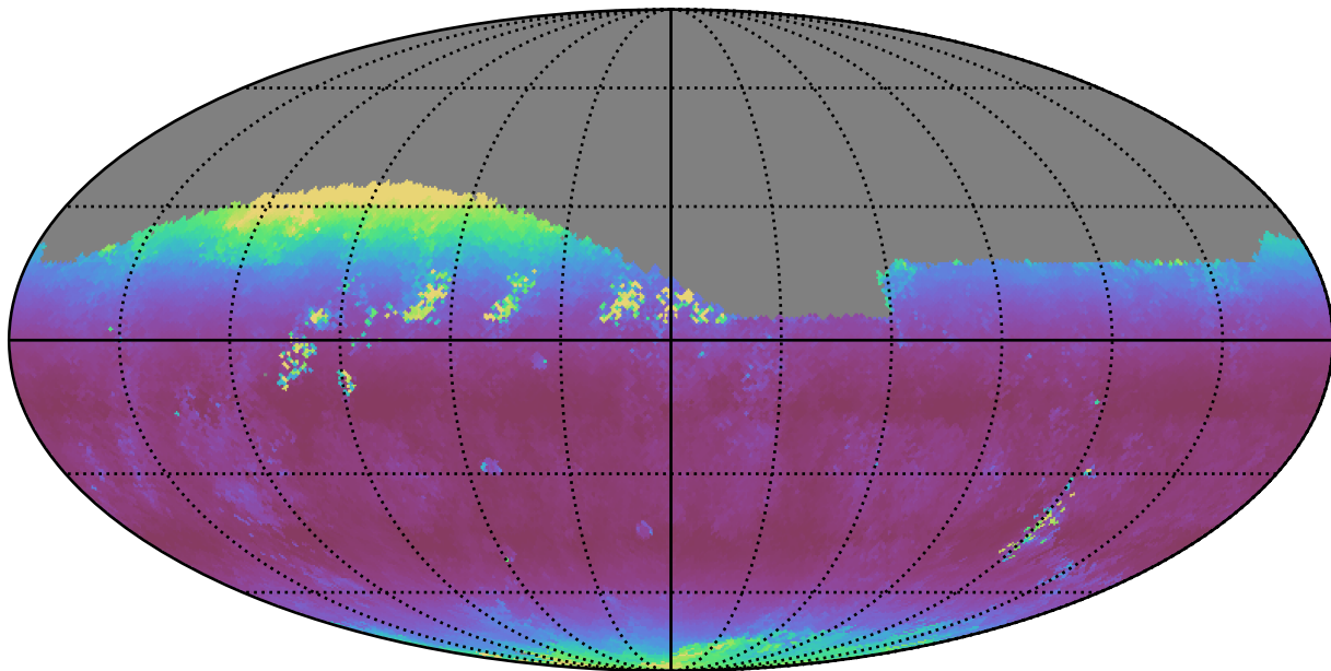
no_magell_roll_v3.4_10yrs Yr 1 r band: Median airmass
