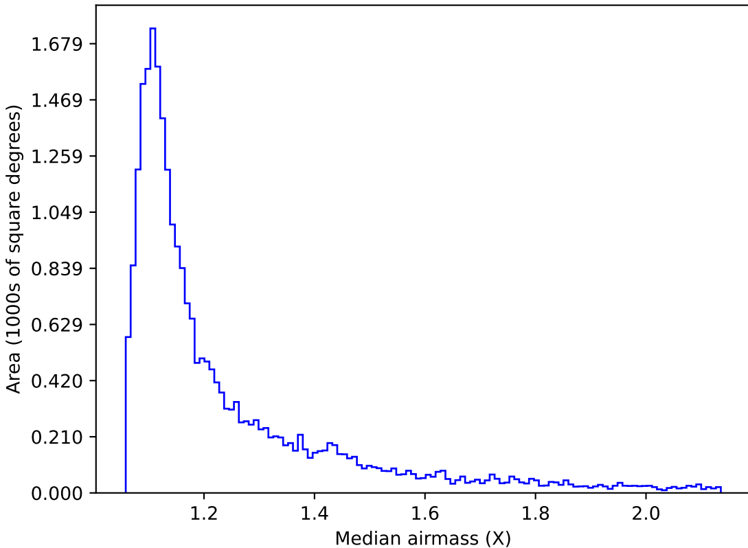
no_magell_roll_v3.4_10yrs Yr 1 r band: Median airmass
