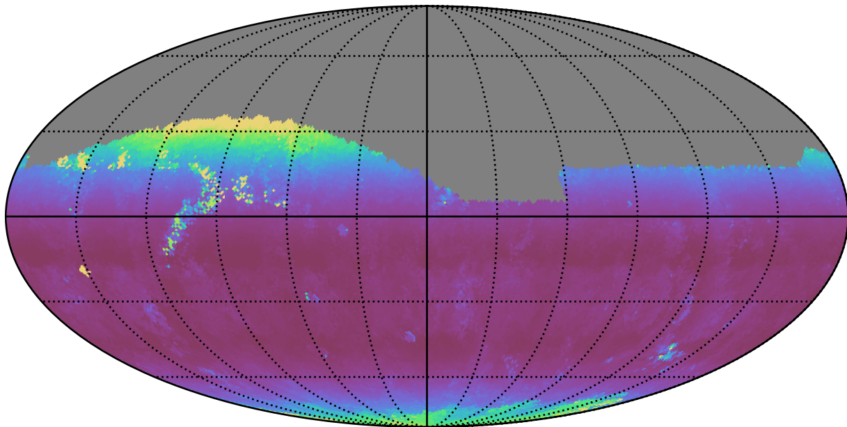
no_magell_roll_v3.4_10yrs Yr 1 i band: Median airmass
