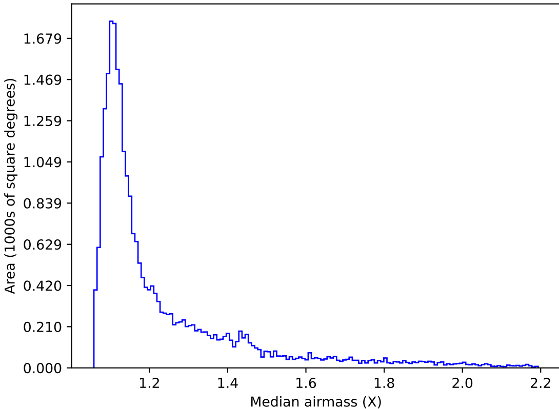
no_magell_roll_v3.4_10yrs Yr 1 i band: Median airmass
