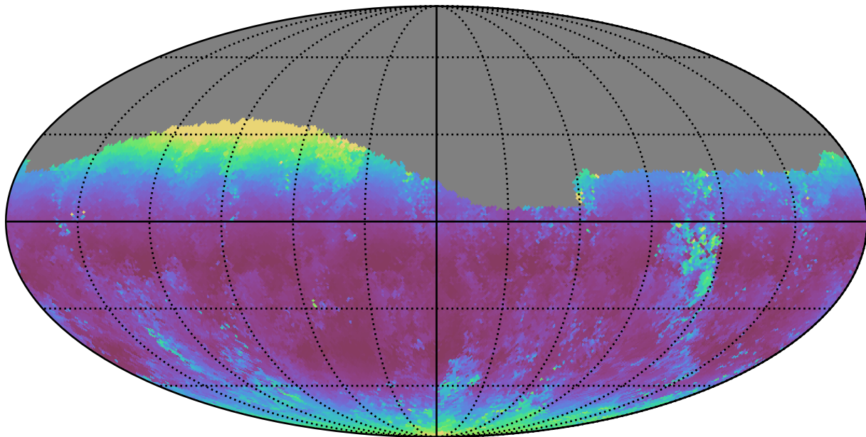
no_magell_roll_v3.4_10yrs Yr 1 g band: Median airmass
