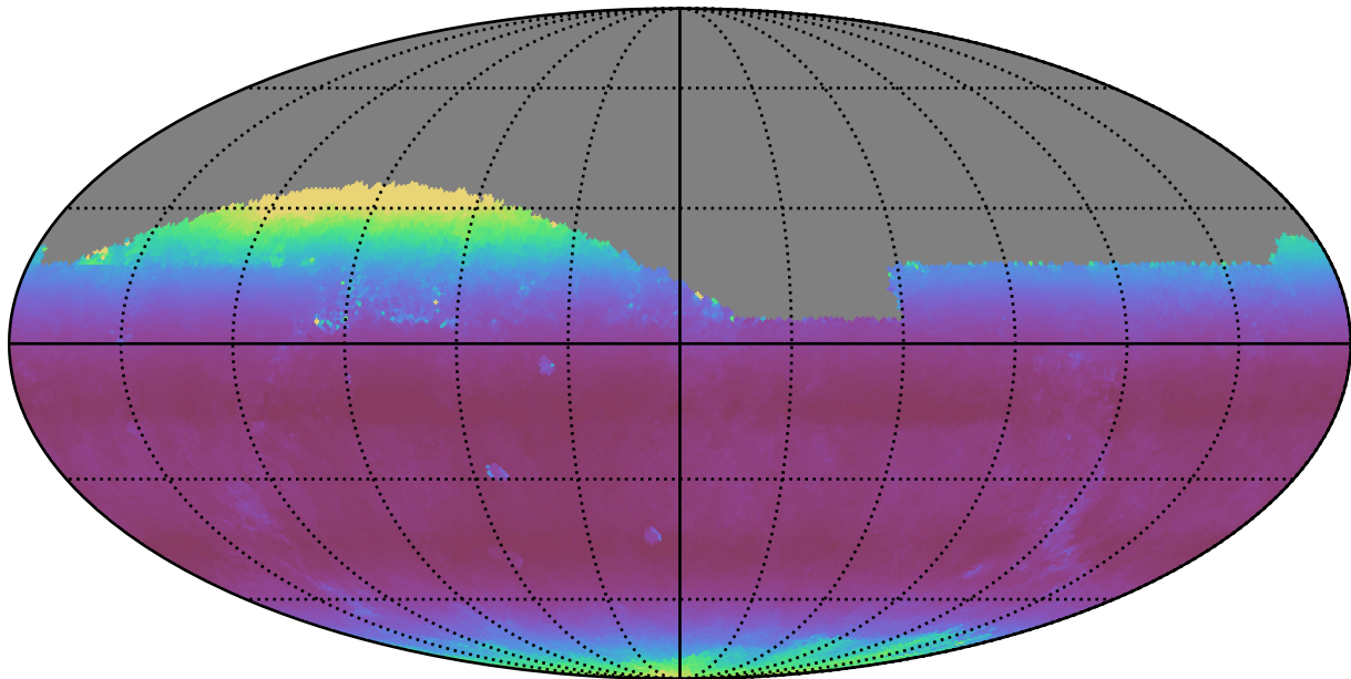
no_magell_roll_v3.4_10yrs Yr 1 all bands: Median airmass
