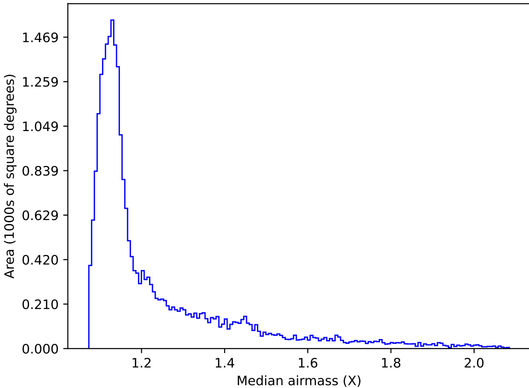
no_magell_roll_v3.4_10yrs Yr 1 all bands: Median airmass
