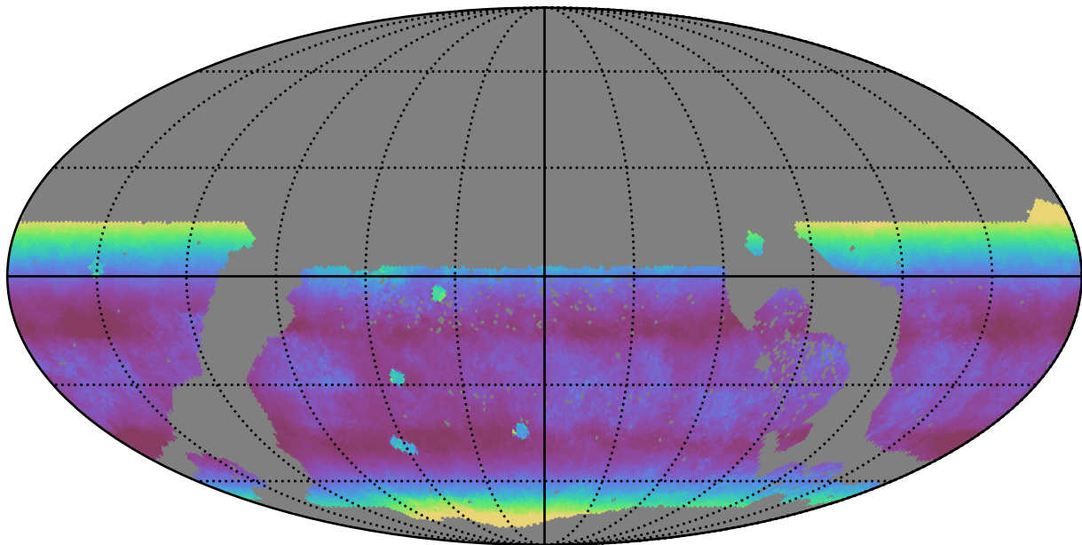
no_magell_roll_v3.4_10yrs WFD z band: Median airmass
