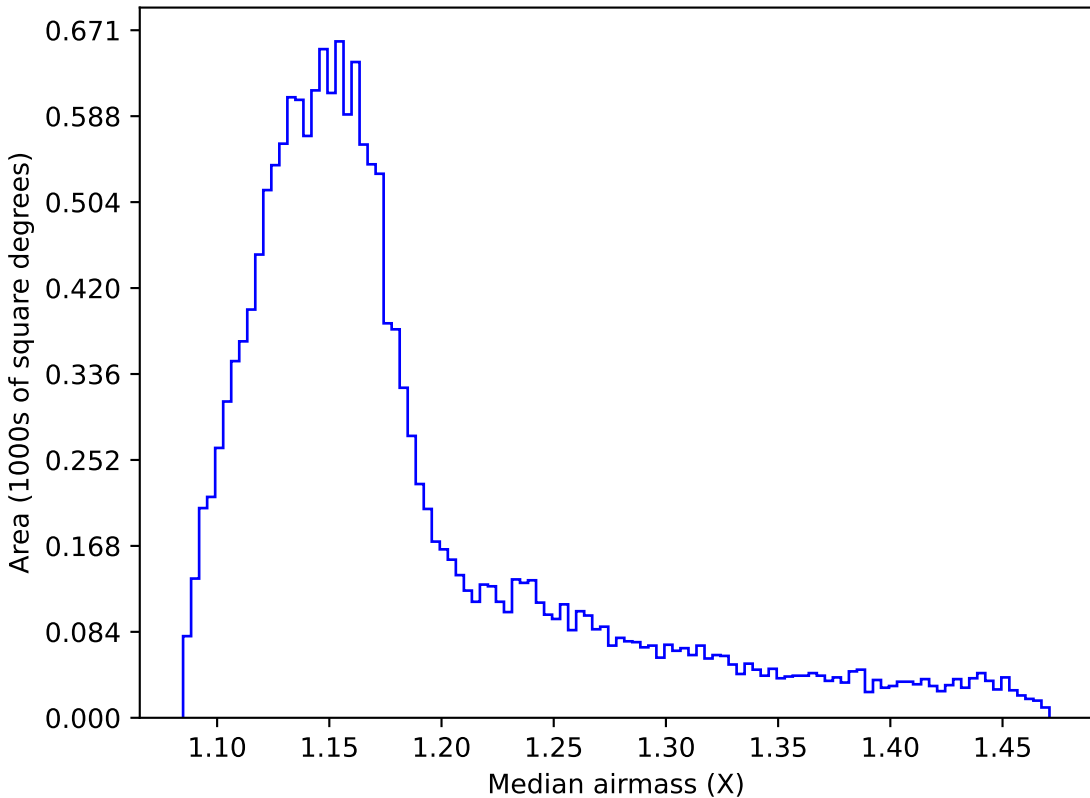
no_magell_roll_v3.4_10yrs WFD z band: Median airmass
