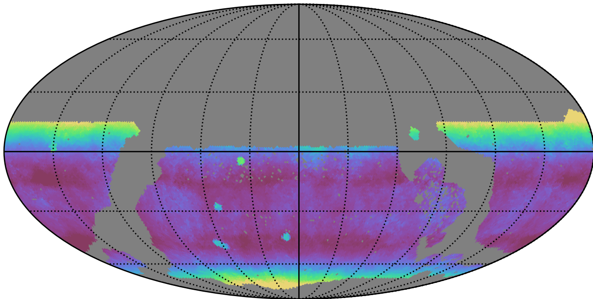
no_magell_roll_v3.4_10yrs WFD y band: Median airmass
