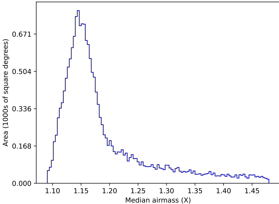
no_magell_roll_v3.4_10yrs WFD y band: Median airmass
