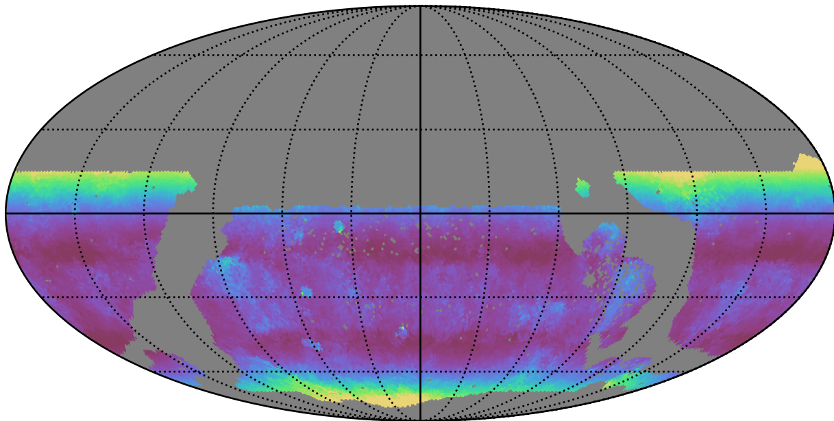
no_magell_roll_v3.4_10yrs WFD u band: Median airmass
