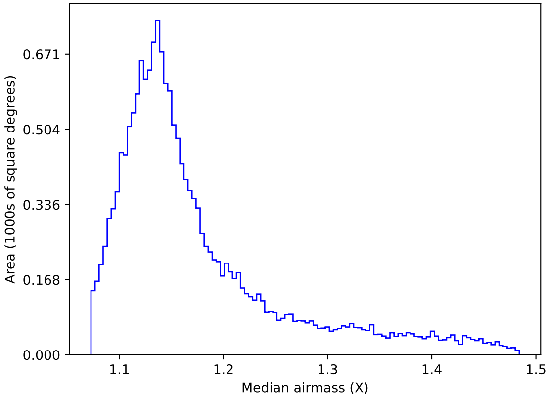
no_magell_roll_v3.4_10yrs WFD u band: Median airmass
