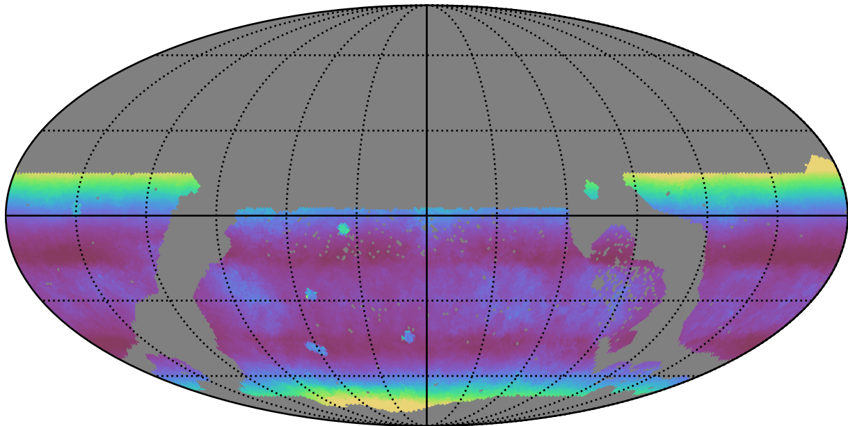
no_magell_roll_v3.4_10yrs WFD r band: Median airmass
