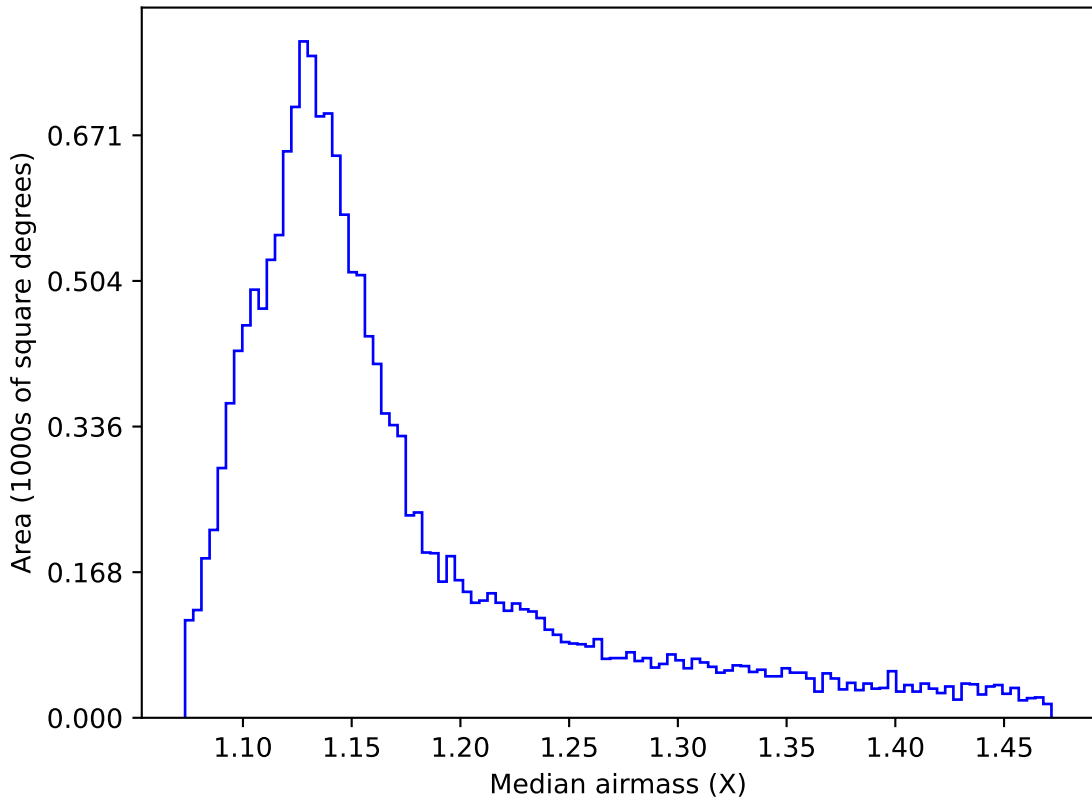
no_magell_roll_v3.4_10yrs WFD r band: Median airmass
