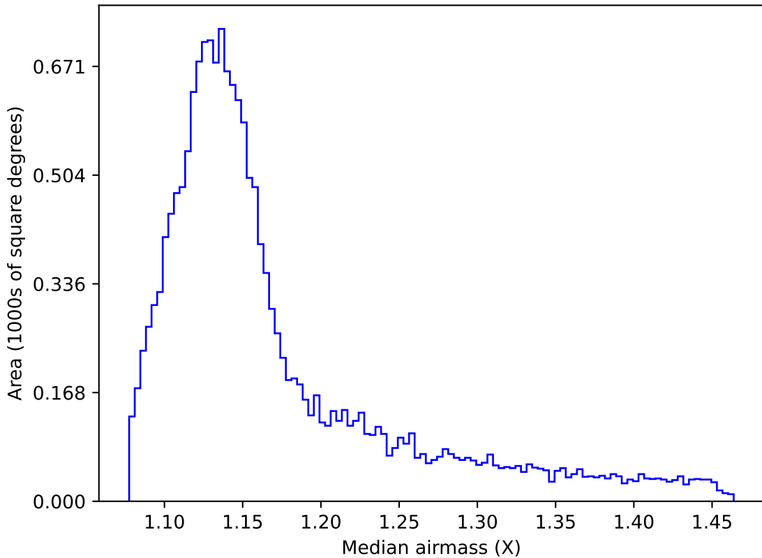
no_magell_roll_v3.4_10yrs WFD i band: Median airmass
