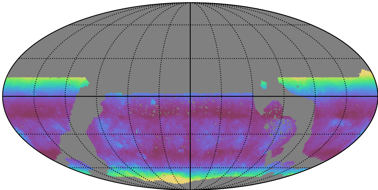
no_magell_roll_v3.4_10yrs WFD g band: Median airmass
