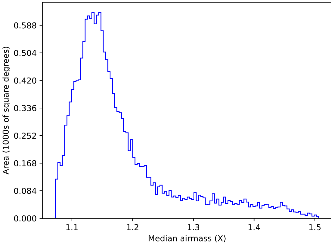
no_magell_roll_v3.4_10yrs WFD g band: Median airmass
