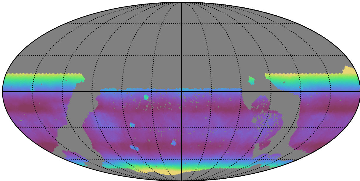
no_magell_roll_v3.4_10yrs WFD all bands: Median airmass
