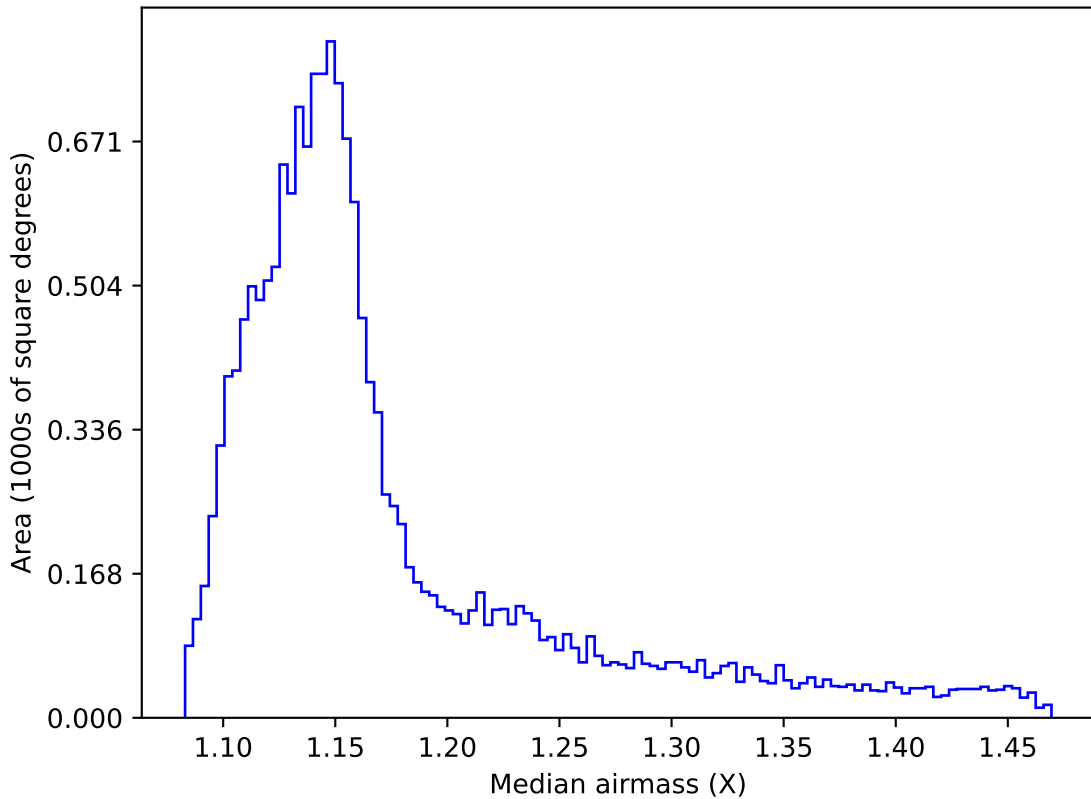
no_magell_roll_v3.4_10yrs WFD all bands: Median airmass
