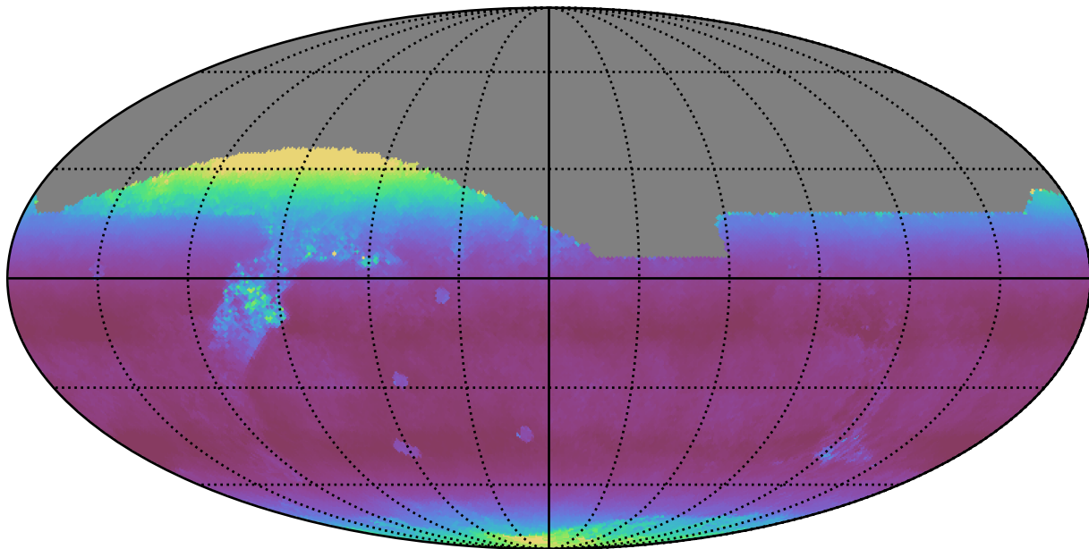
no_magell_roll_v3.4_10yrs All sky z band: Median airmass
