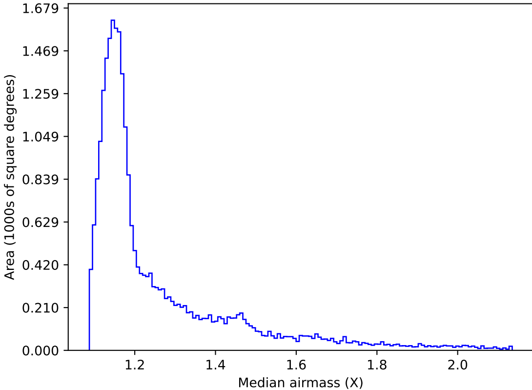
no_magell_roll_v3.4_10yrs All sky z band: Median airmass
