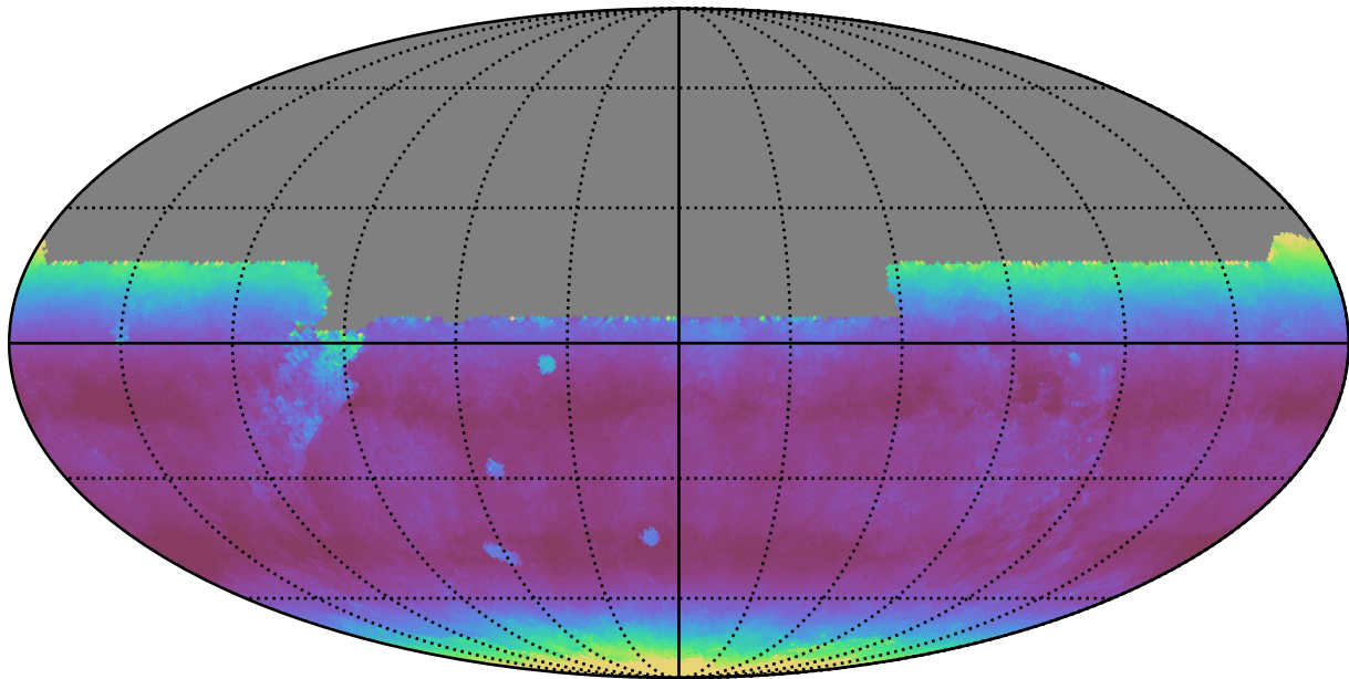
no_magell_roll_v3.4_10yrs All sky y band: Median airmass
