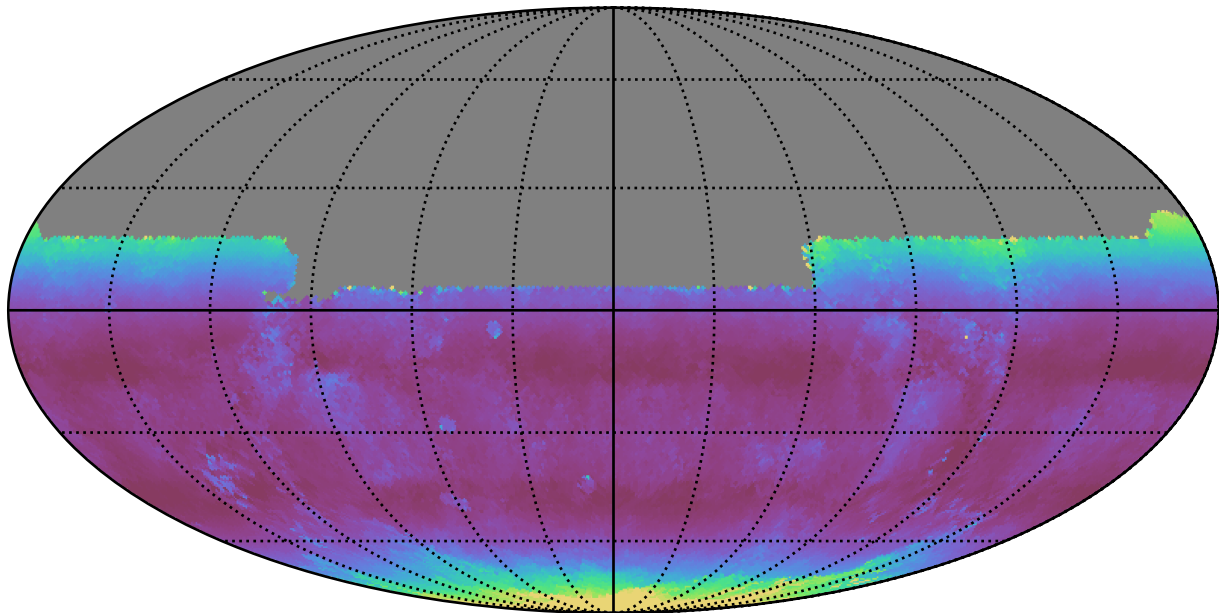
no_magell_roll_v3.4_10yrs All sky u band: Median airmass
