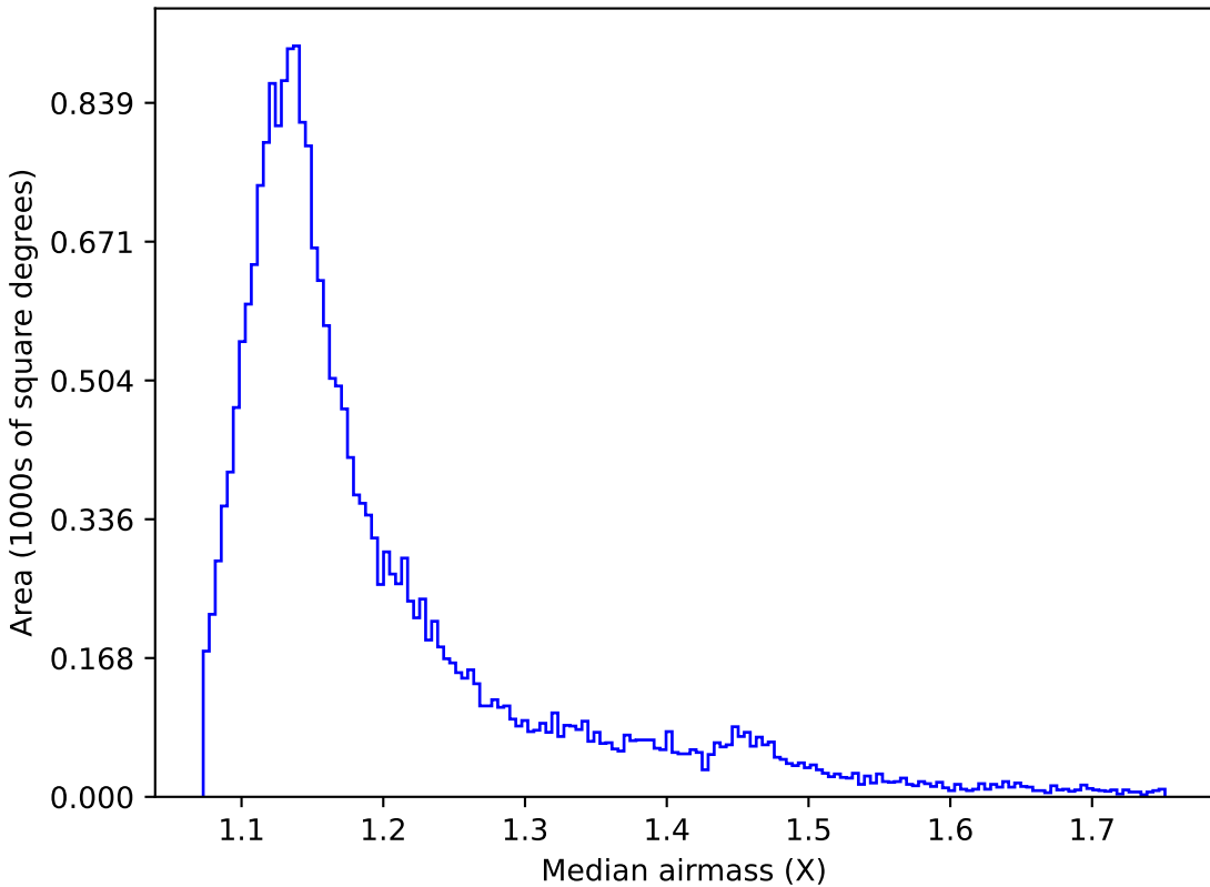
no_magell_roll_v3.4_10yrs All sky u band: Median airmass
