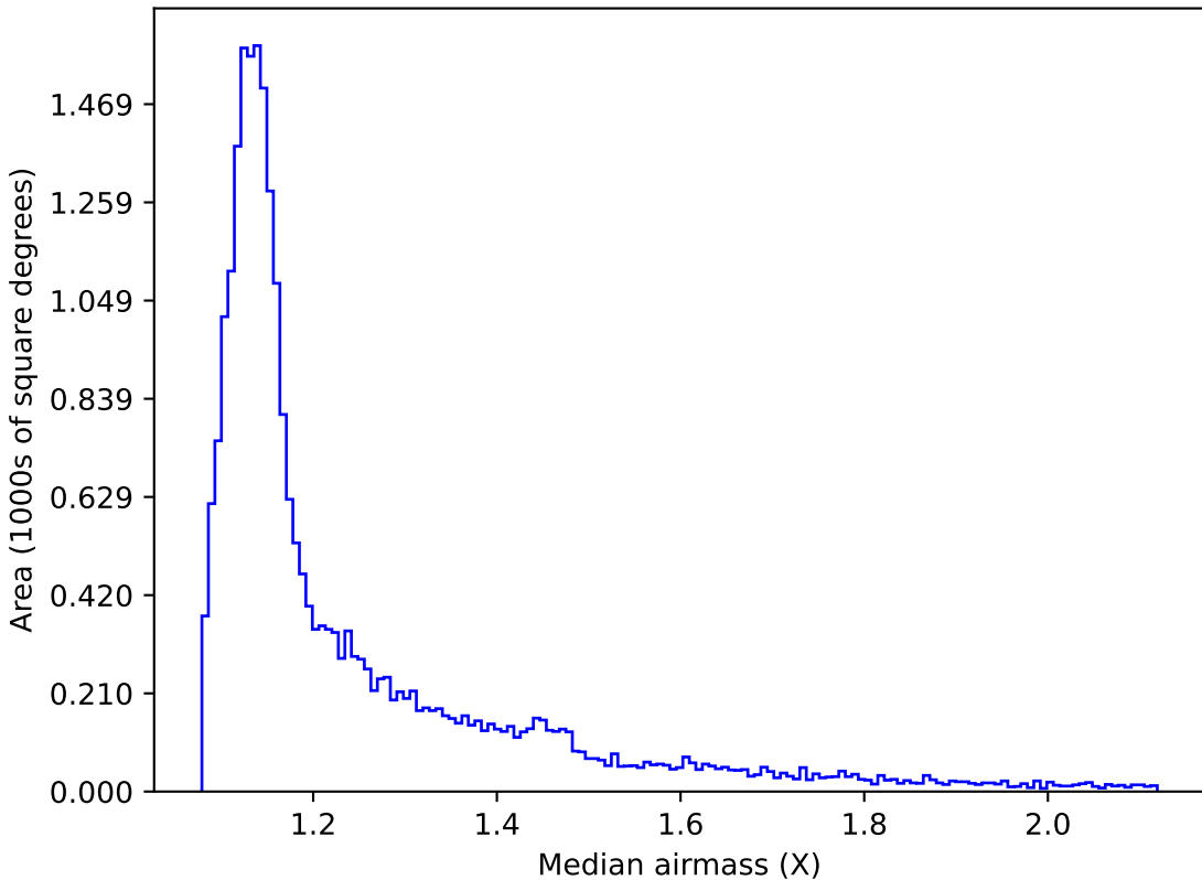
no_magell_roll_v3.4_10yrs All sky i band: Median airmass
