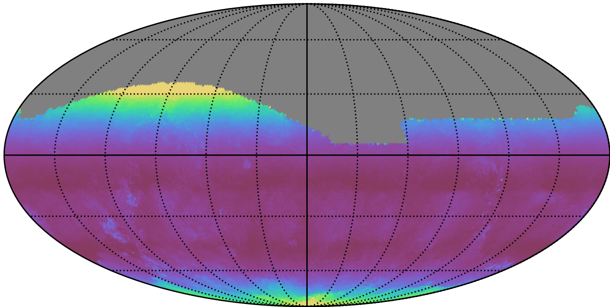
no_magell_roll_v3.4_10yrs All sky g band: Median airmass
