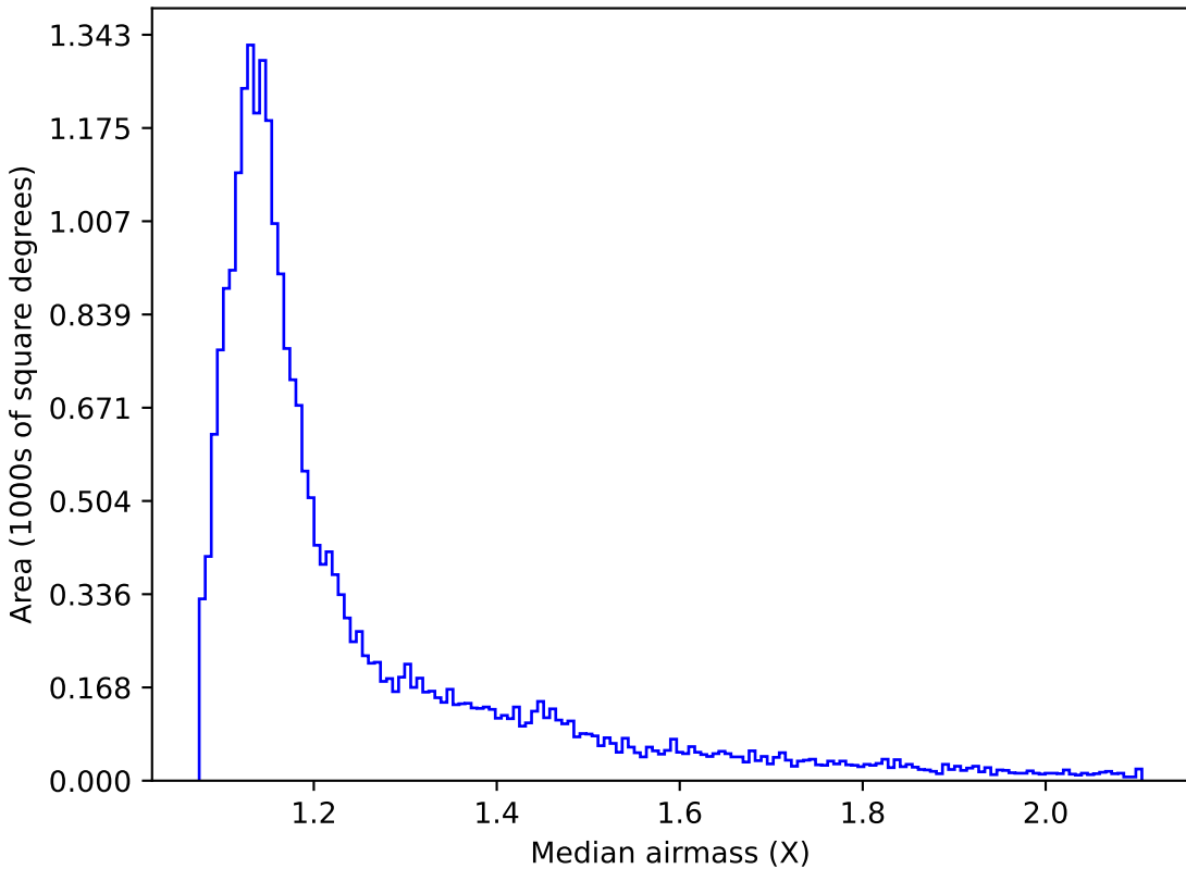
no_magell_roll_v3.4_10yrs All sky g band: Median airmass
