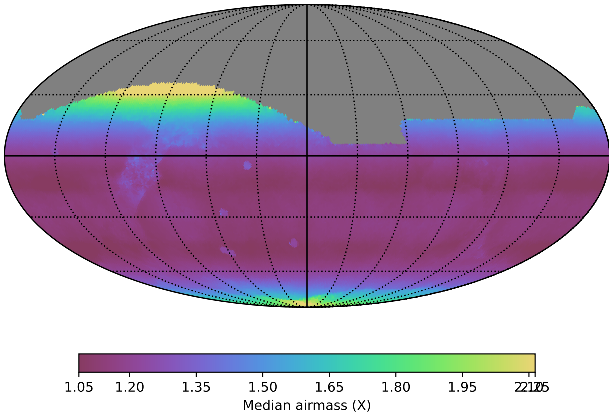
no_magell_roll_v3.4_10yrs All sky all bands: Median airmass
