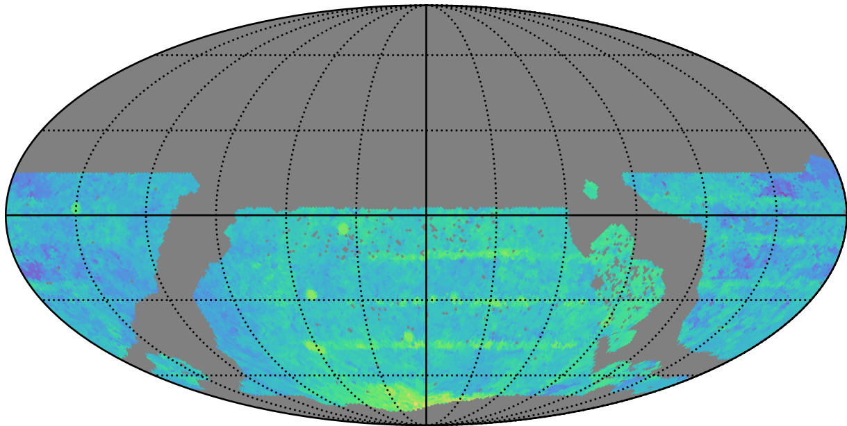
no_magell_roll_v3.4_10yrs WFD z band: Median Season Length
