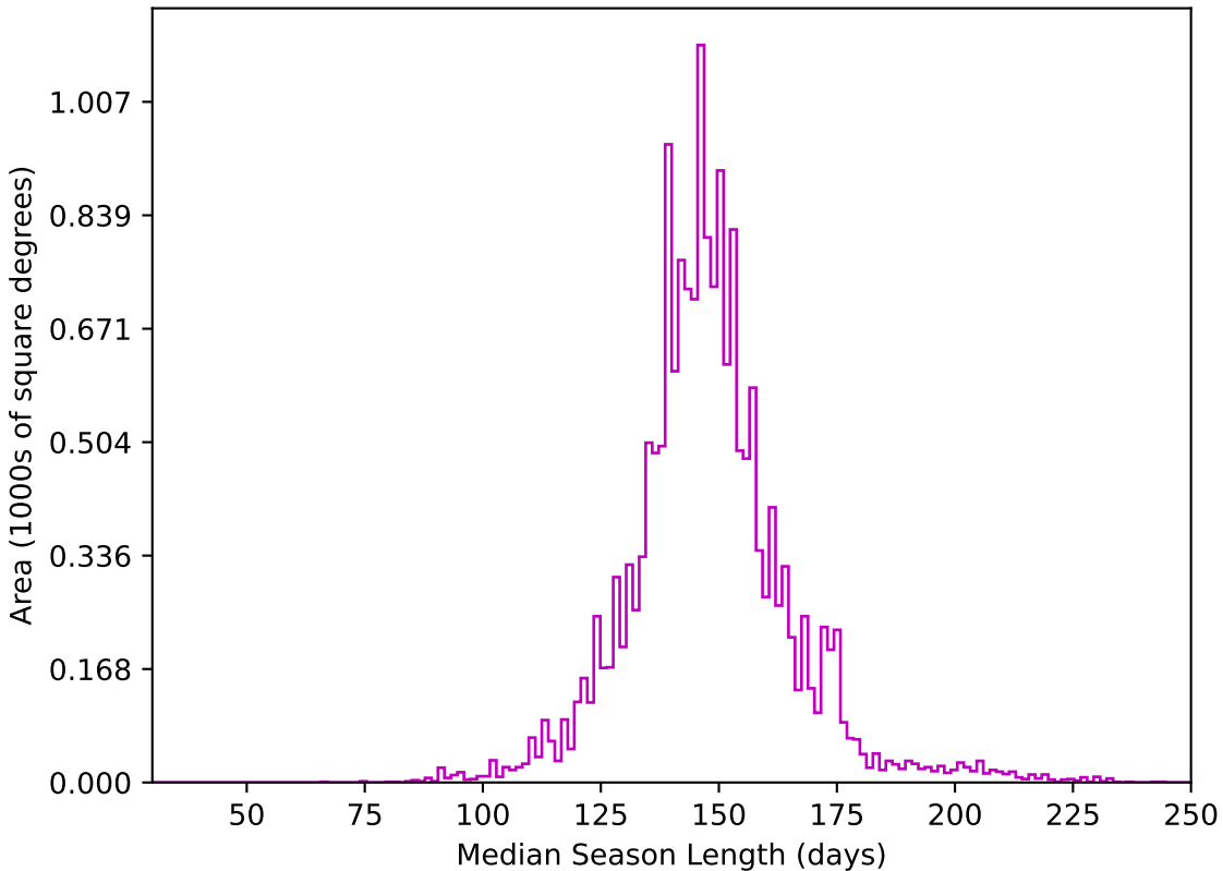
no_magell_roll_v3.4_10yrs WFD z band: Median Season Length
