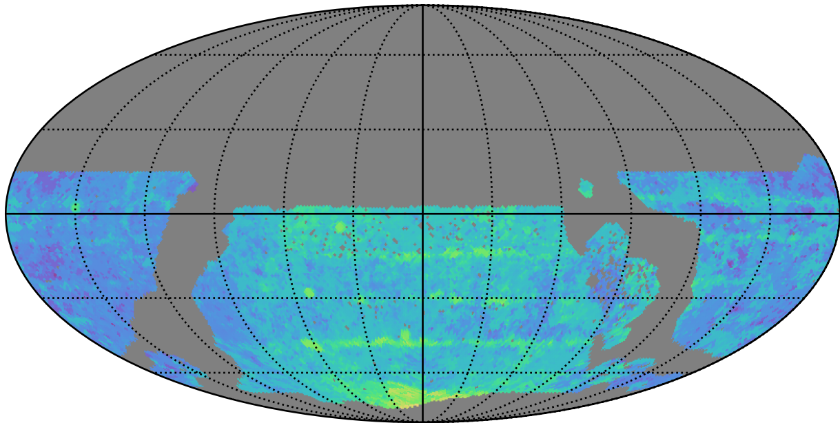
no_magell_roll_v3.4_10yrs WFD y band: Median Season Length
