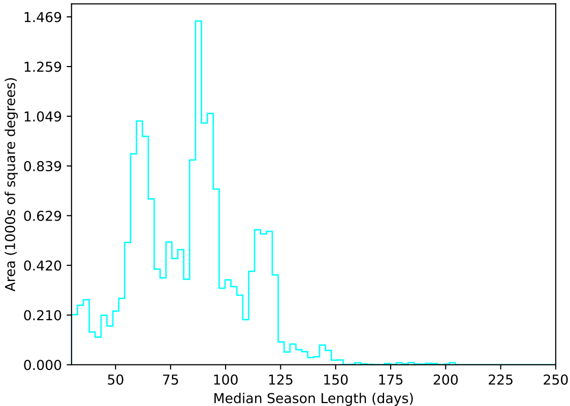
no_magell_roll_v3.4_10yrs WFD u band: Median Season Length
