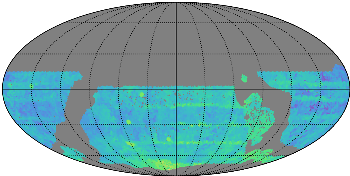
no_magell_roll_v3.4_10yrs WFD r band: Median Season Length
