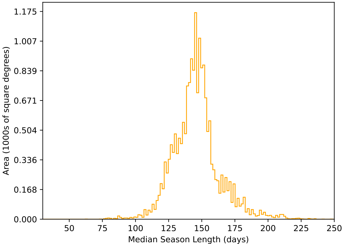
no_magell_roll_v3.4_10yrs WFD r band: Median Season Length
