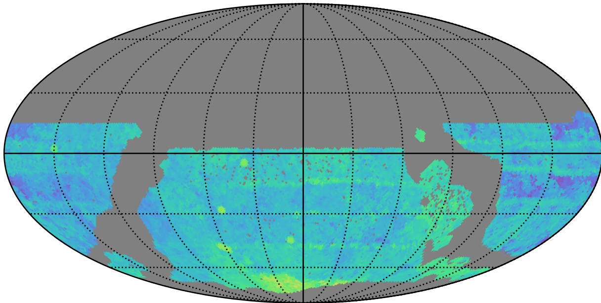
no_magell_roll_v3.4_10yrs WFD i band: Median Season Length
