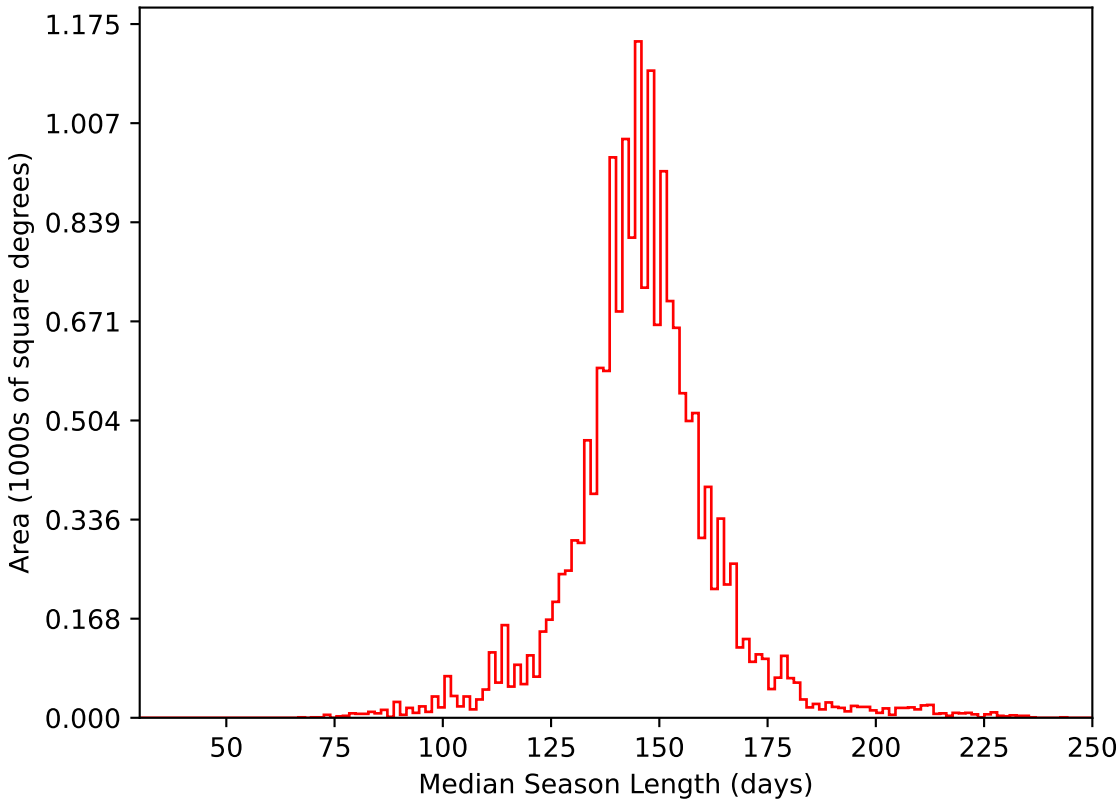
no_magell_roll_v3.4_10yrs WFD i band: Median Season Length
